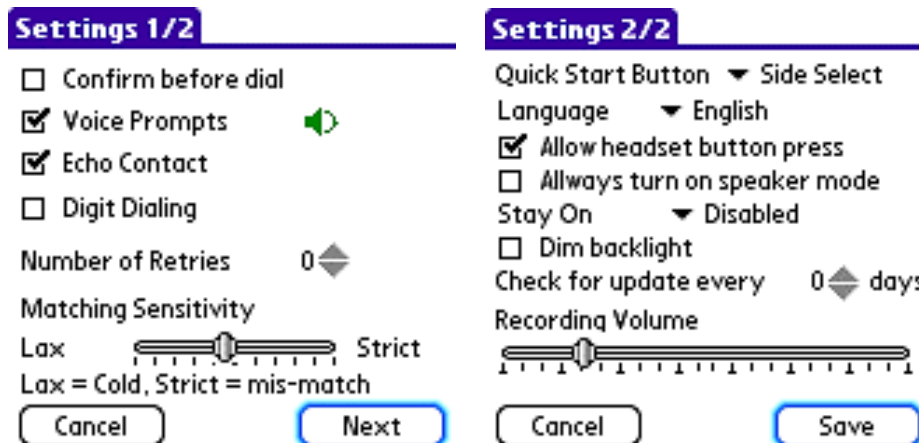
Diagram 6: Settings Screens
